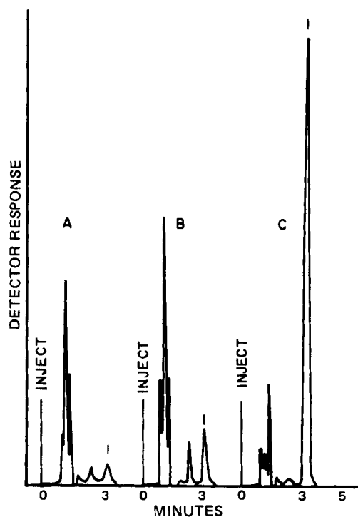
Figure 2 —Sample chromatograms where peak 1 is from furosemide. Key: A, solution of 1 (0.05%) in pH 5 buffer with 0.1% sodium metabisulfite after 170 days of storage at room temperature; B, same as A except that pH 6 buffer was used; and C, same as A except that pH 9 buffer was used.
